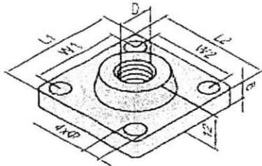
9.1. Leveling Foot - Fixed Foot M12 X 70
