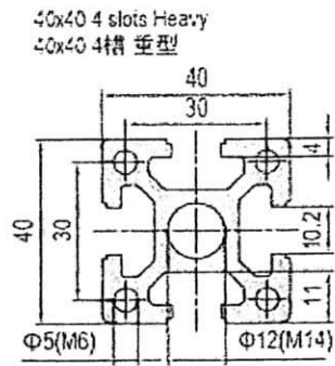
1.1. X-Section : 40 x 40 Heavy
