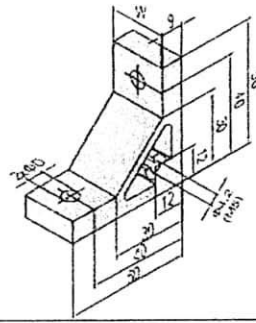
7.1. Angle Profile Bracket 40/40
