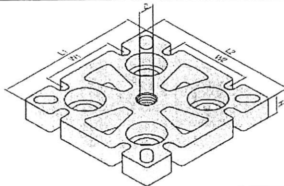
9.4. Mounting Plate X Section 80 x 80 (M12)
