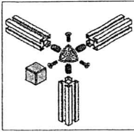
6.4. Cubic Connector 40/3
