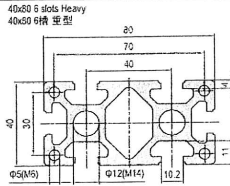
1.2. X-Section : 40 x 80 Heavy
