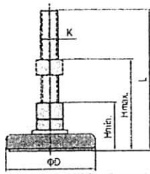
9.1. Leveling Foot - Fixed Foot M12 X 70
