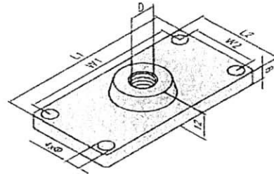
9.3. Mounting Plate X Section 40 x 80 (M12)
