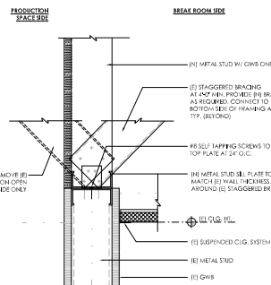
THRU-GRID INTERIOR PARTITION EXTENSION METAL STUD
