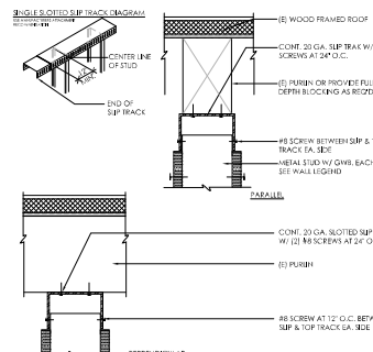
FULL HEIGHT WALL TERMINATION AT WOOD FRAMED STRUCTURE
