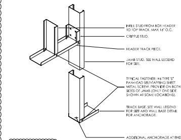
TYPICAL DOOR OPENING FRAMING NON-BEARING SPANS UP TO 4'-0"
