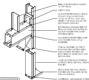
TYPICAL DOOR OPENING FRAMING SPANS 4'-0" TO 12'-0" 1
